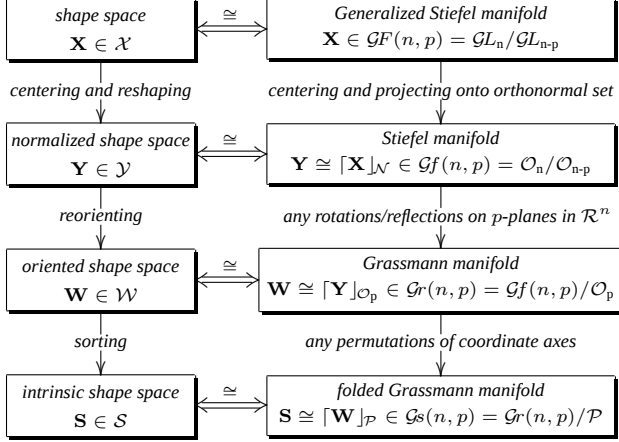
Fig. 1. Shape space reduction
